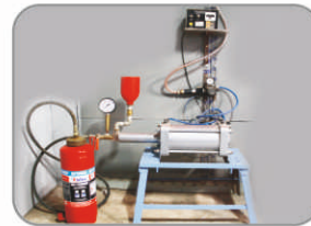
Pressure Cyclic Test
